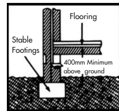
Platform construction
