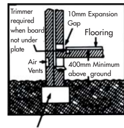
Fitted floor
