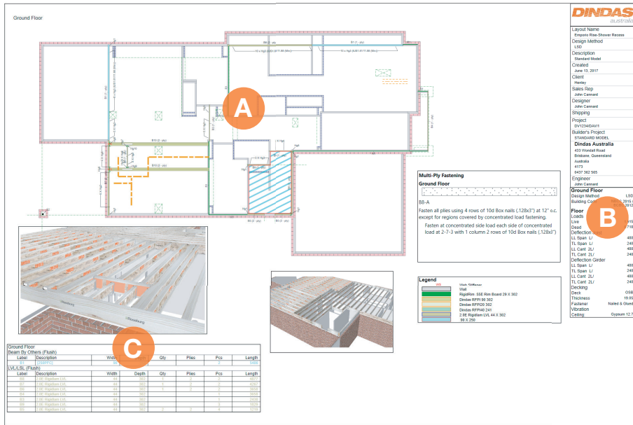
A. Cost-effective joist selection B. Take-off list C. Bracket selection *
