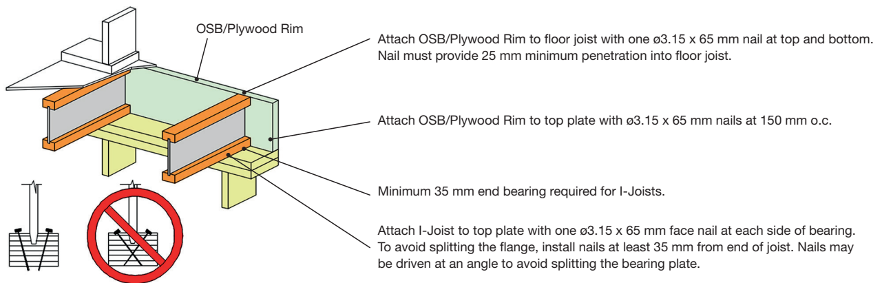
Diagram 1B.1 Rim Board at Exterior Wall (perp. joists)
