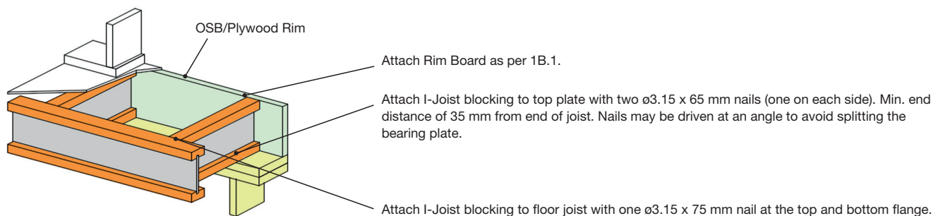
Diagram 1B.2 Exterior End Wall Support (perp. blocking)
