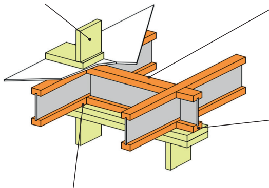
Attach I-Joist to top plate as per 1B.1.
