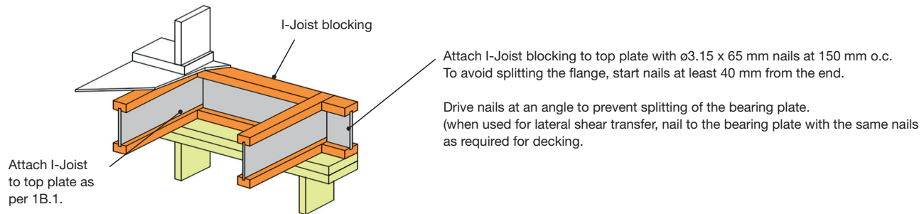
Diagram 1B.1 Rim Board at Exterior Wall (perp. joists)
